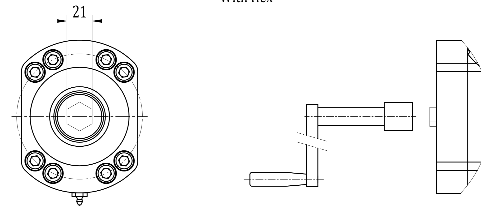
A向/A View
