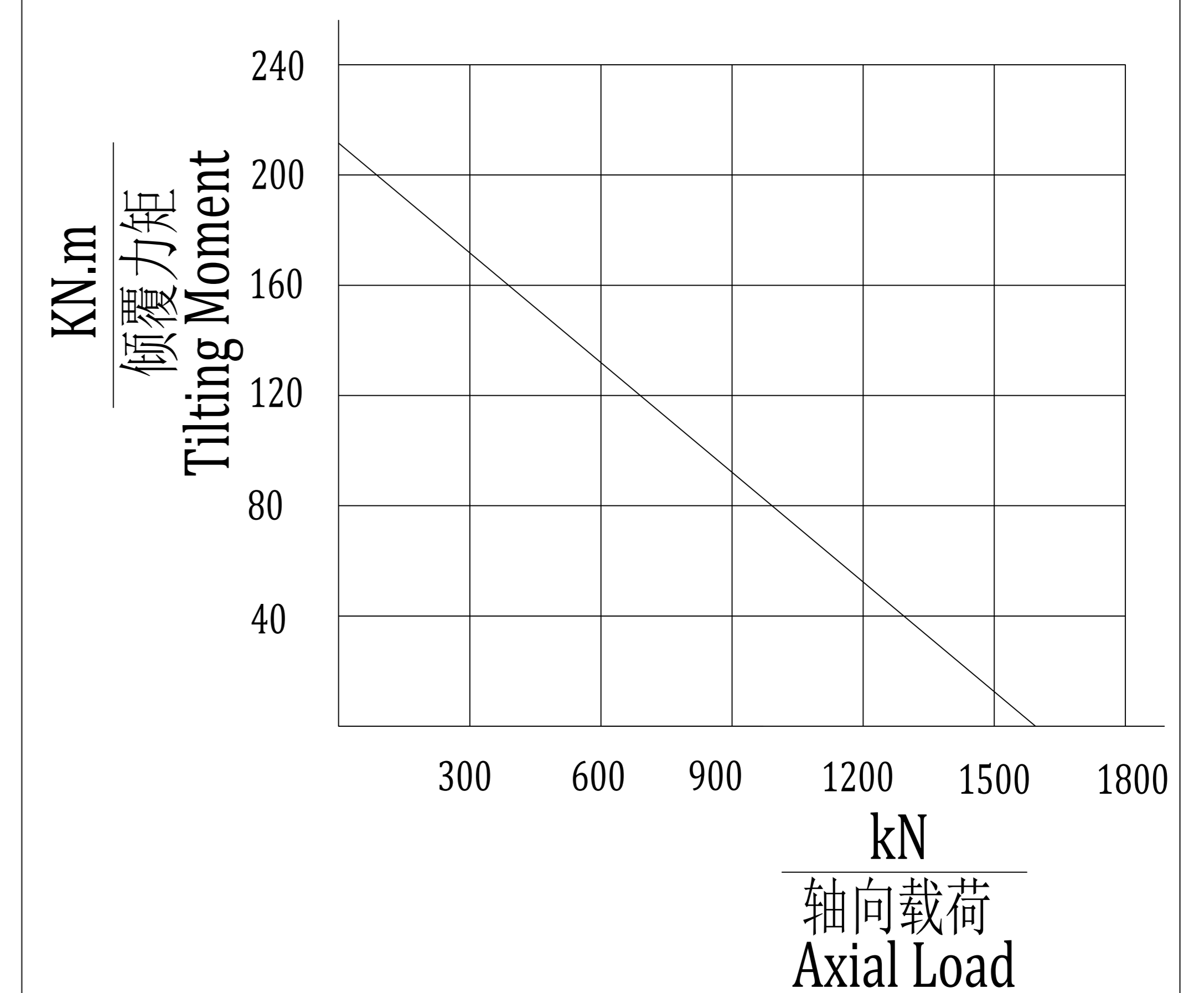
承载力矩图 MOMENT LOAD CHART 轴向载荷 & 倾覆力矩 Axial Load & Tilting Moment
